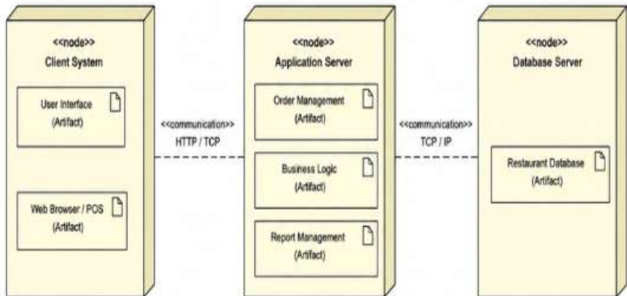
Deployment Diagram - Restaurant Management System
